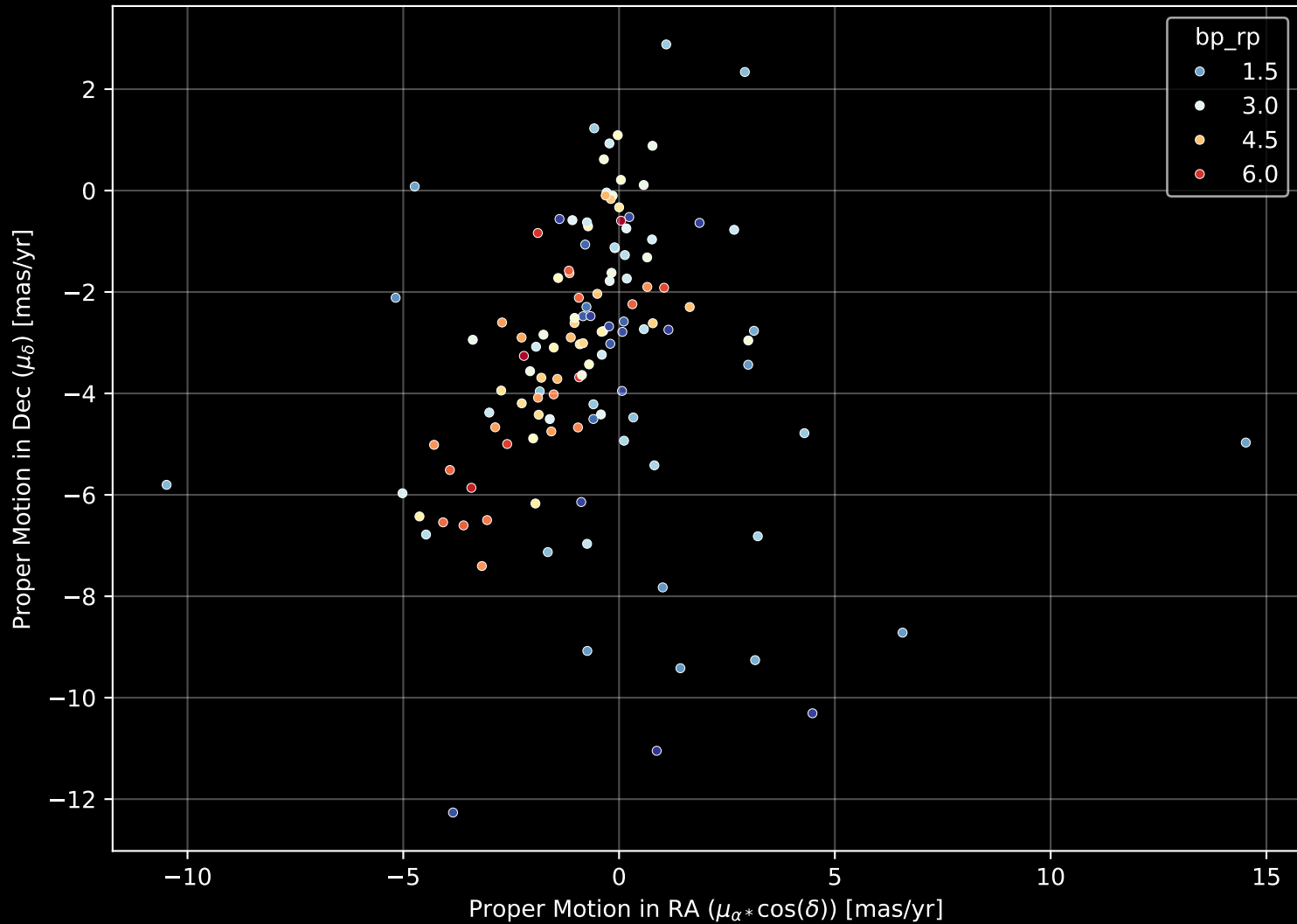
APOGEE DR17 Field: [018+00] Proper Motion Diagram (n= 124)
