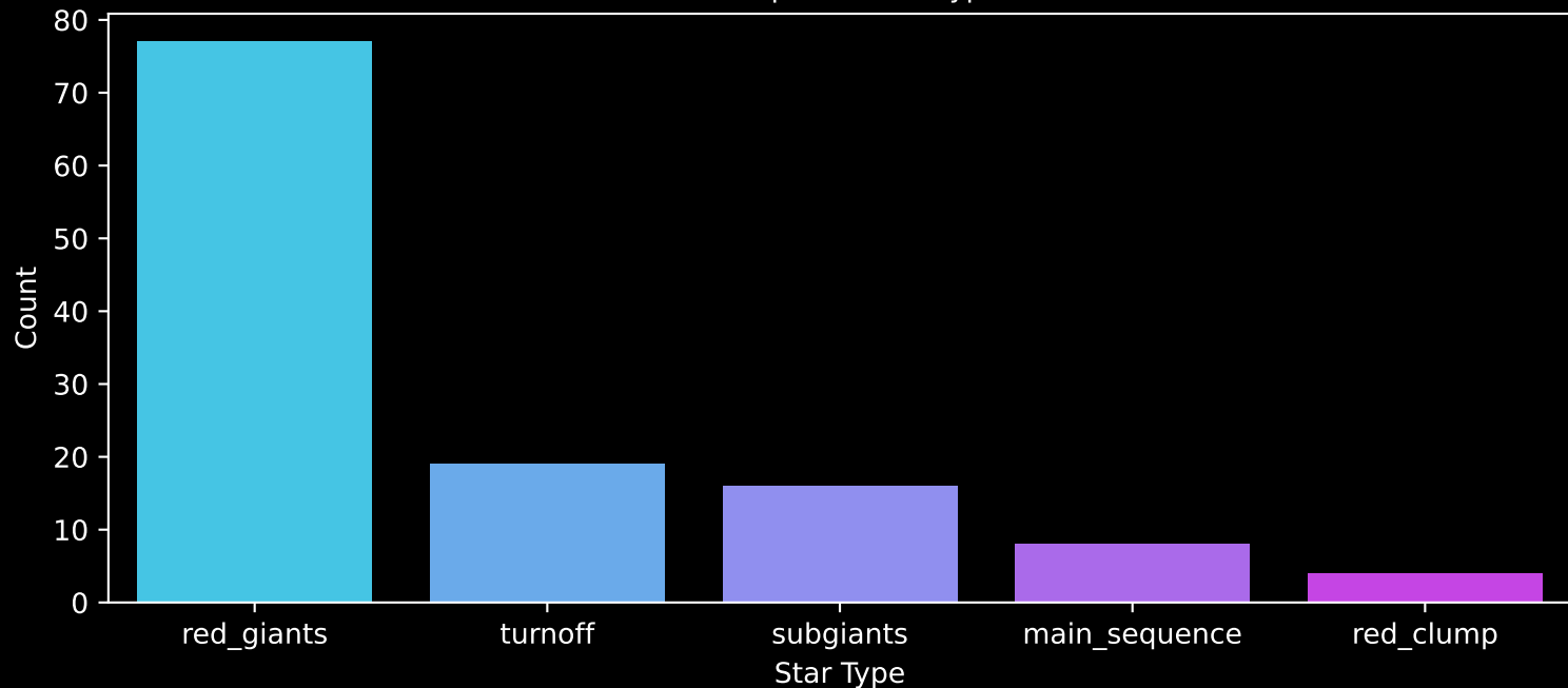
APOGEE DR17 Field: [018+00] Count plot of Star Type
