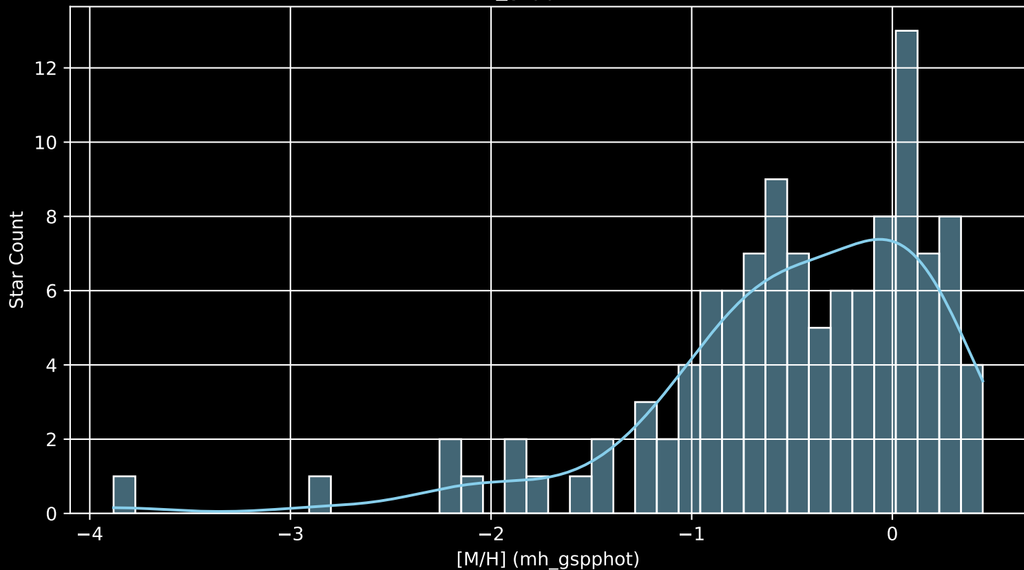
APOGEE DR17 Field: [018+00 [M/H] (mh_gspphot) (n= 112)
