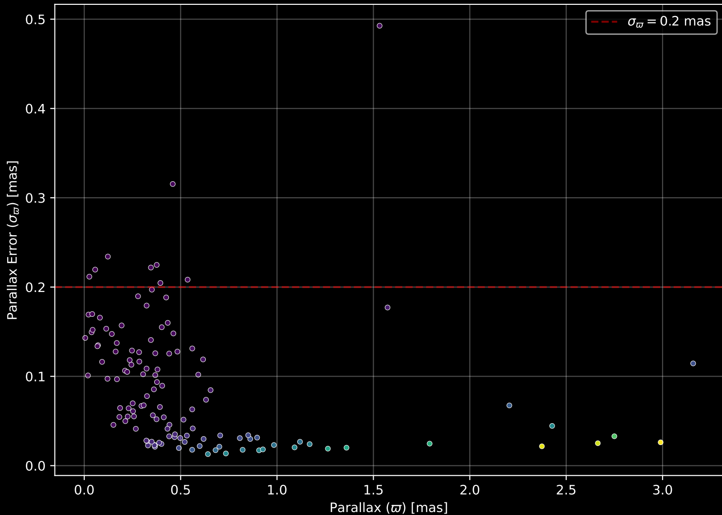
APOGEE DR17 Field: [018+00] Parallax Quality (n= 124)
