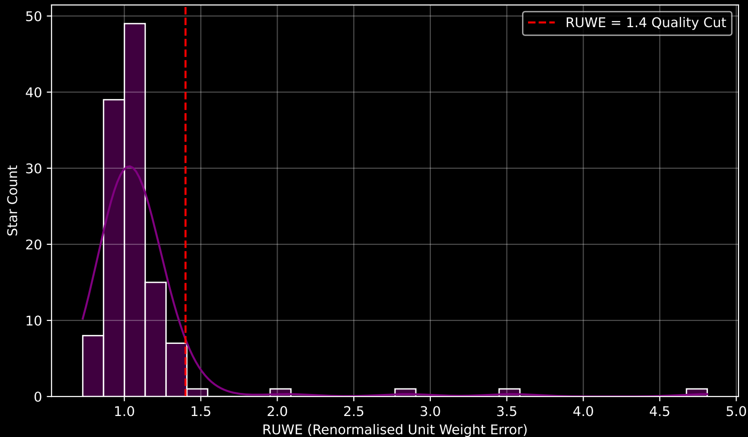
GAPOGEE DR17 Field [018+00] RUWE Distribution (n= 123)
